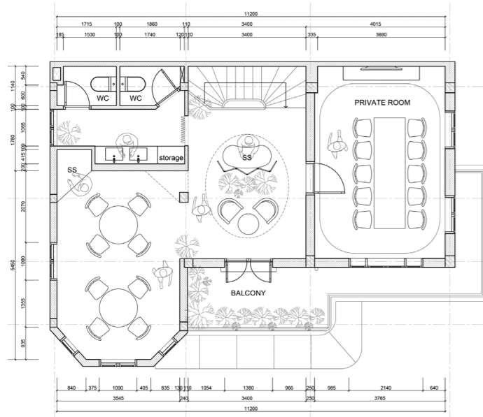
1. Project plan construction drawing
